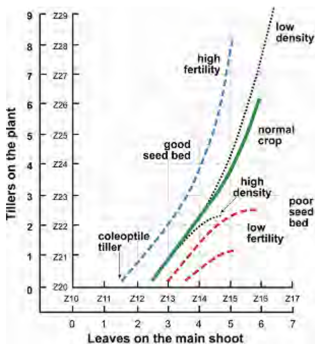
Figure 8. Tillering as a function of leaves per plant and being dependent on management and variety. Low density, normal crop and high density show tillering in 70, 150 and 375 plants/m 2 stands, respectively. The low density trajectory may also be followed for early sown very late (winter) wheat and may lead to 14 tillers at Z17 and 30 tillers at Z19.
